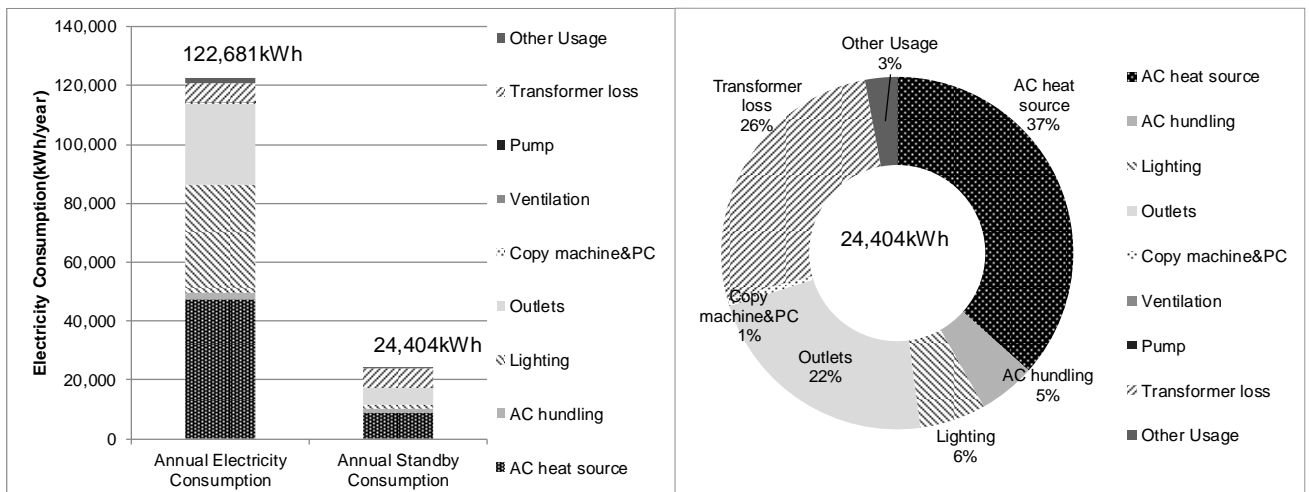
Figure 5 The annual standby power consumption (City hall B)
