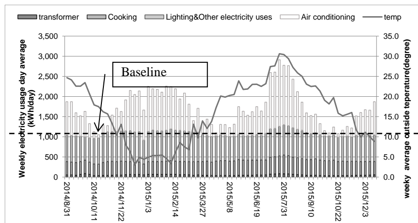
Figure 2 the weekly day average of the electricity consumption and the baseline (Restaurant A)
