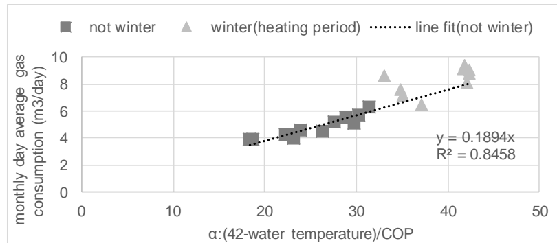
Figure 3 the monthly day average gas consumption and the line fitting
