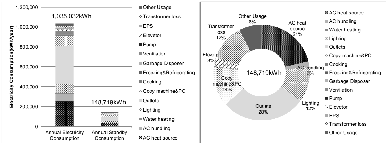
Figure 4 The annual standby power consumption of purpose (City hall A)
